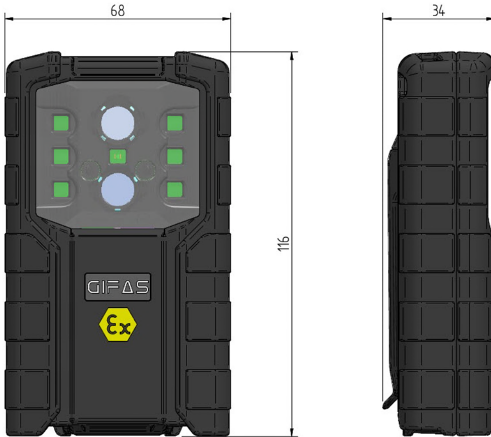
image 4: dimensions TorchLED 2 Ex
